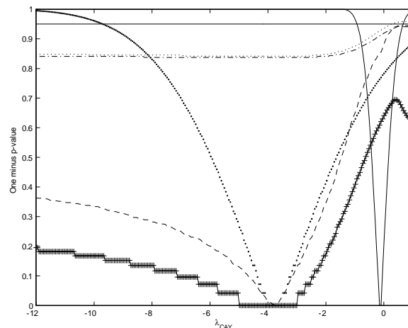
Figure 6.2: p -value plot \lambda_{cay}
