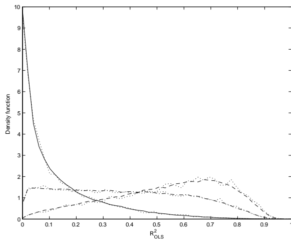
Figure 3.1. Density functions of R^2_{OLS}
