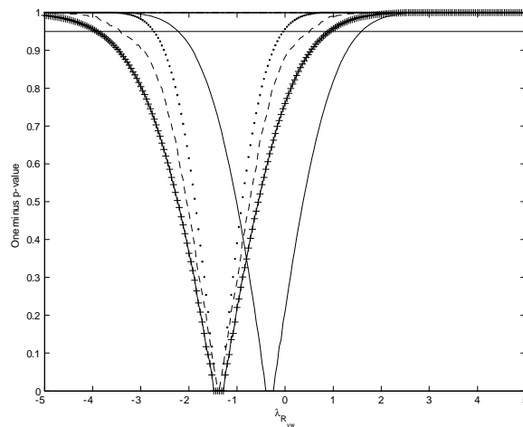
Figure 6.4: p -value plot \lambda_{r_{vw}}
