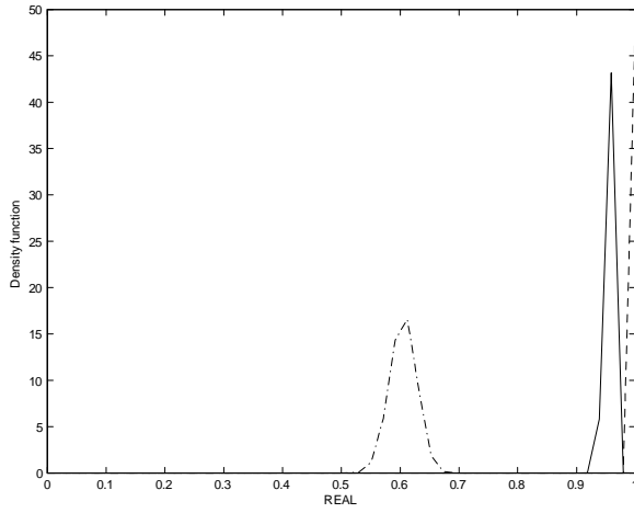
Figure 4.3. Density functions FACCHECK
