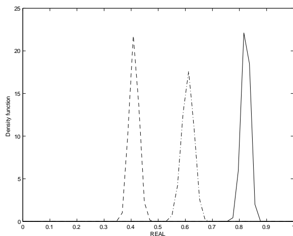
Figure 1.3. Density functions FACCHECK
