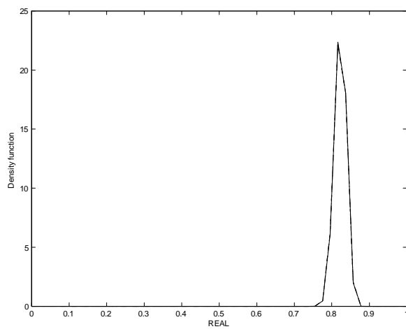
Figure 3.3. Density functions FACCHECK
