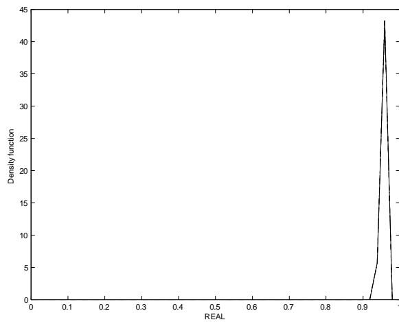
Figure 2.3. Density functions FACCHECK
