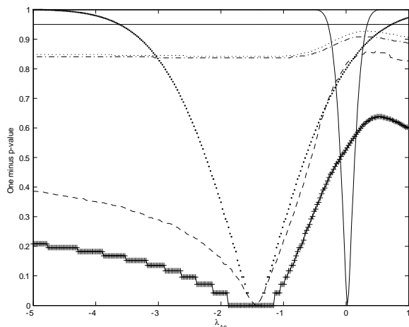
Figure 6.1: p -value plot \lambda_{\Delta c}
